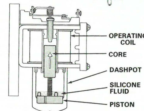
Cross sectional view. Moving parts are shaded.
