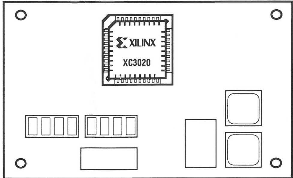
Demonstration Board with XC3020 Logic Cell Array
