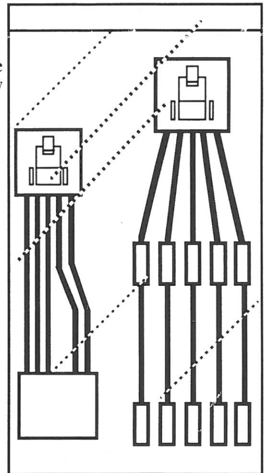
Demonstration Board with XC3020 Logic Cell Array
