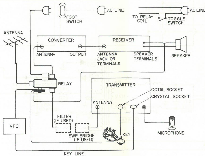
FIG.4 CONNECTIONS FOR PHONE AND CW OPERATION
