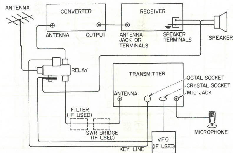
FIG.3 CONNECTIONS FOR PHONE OPERATION
