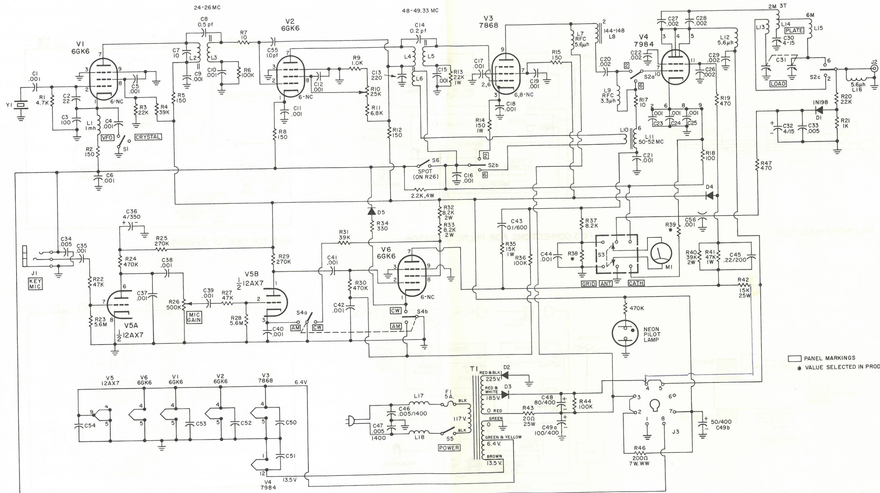
AMECO MODEL TX-62 TRANSMITTER
