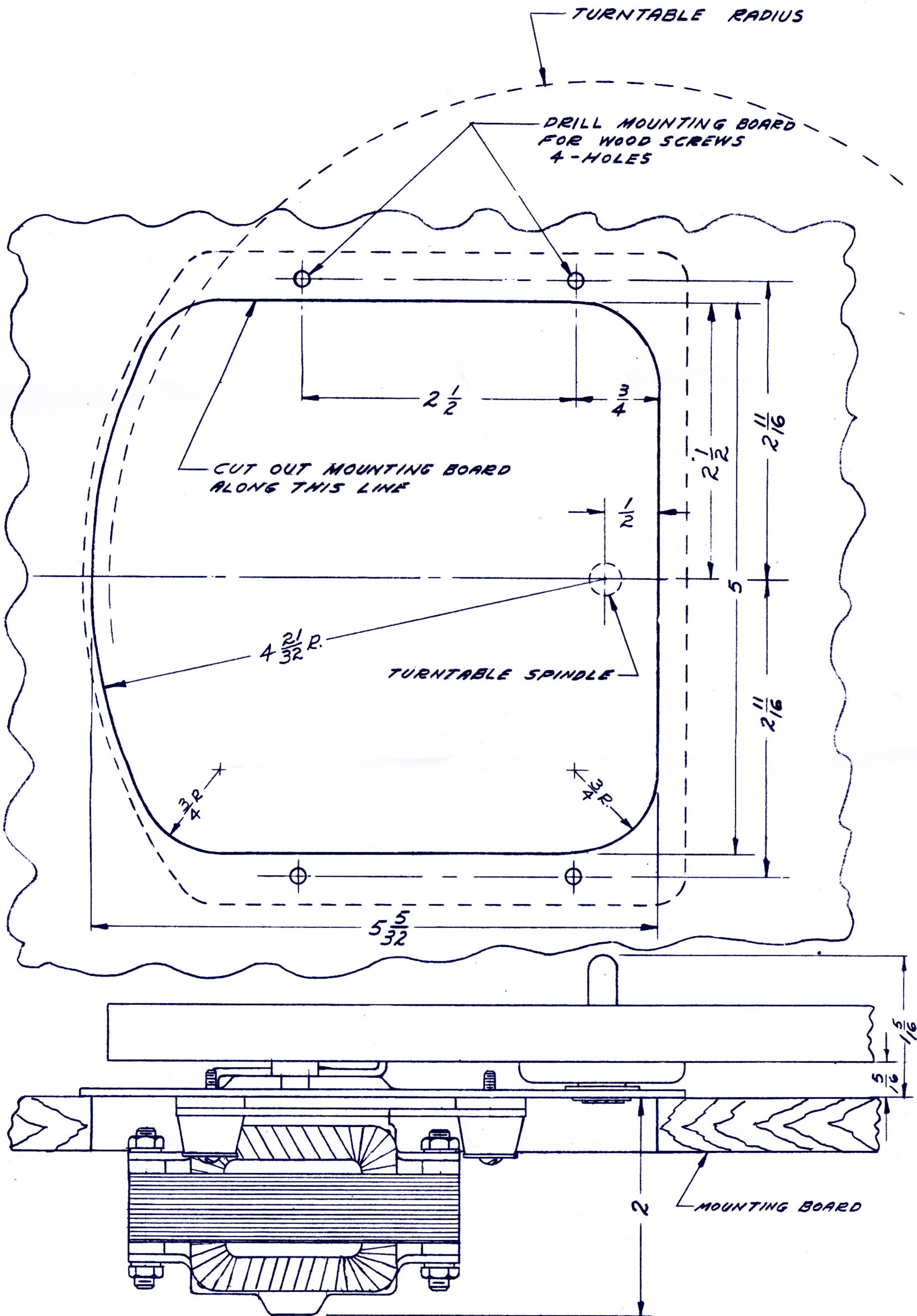
TEMPLATE & MOUNTING DETAILS FOR M-15 MOTOR & TURNTABLE ASSEMBLY
