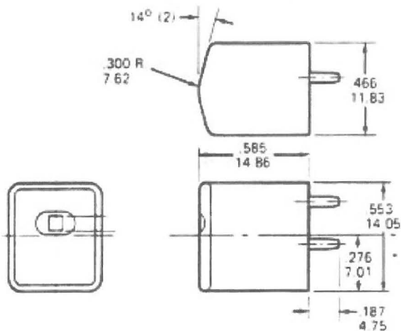
43G 'G' SIZE DIMENSIONS
