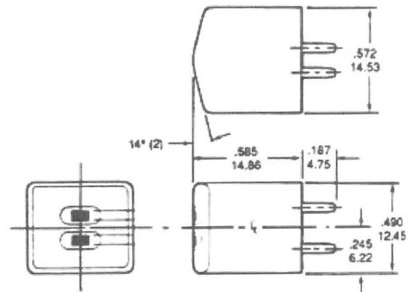
41B "B" SIZE DIMENSIONS
