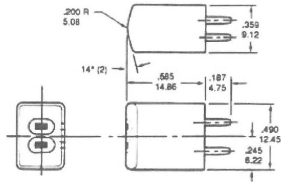
42C 'C' SIZE DIMENSIONS
