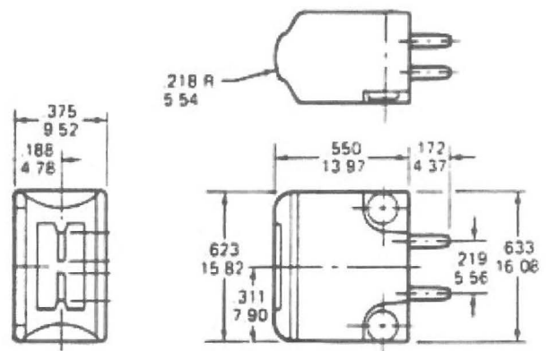
44LE 'LE' ERASE DIMENSIONS
