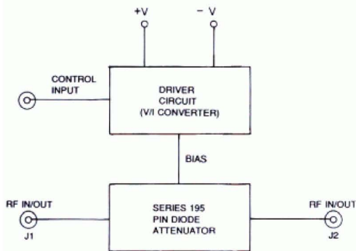
Fig. 1-Series D195, block diagram
