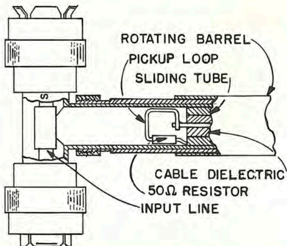
Figure 1. Cutaway view of adjustable attenuator.
