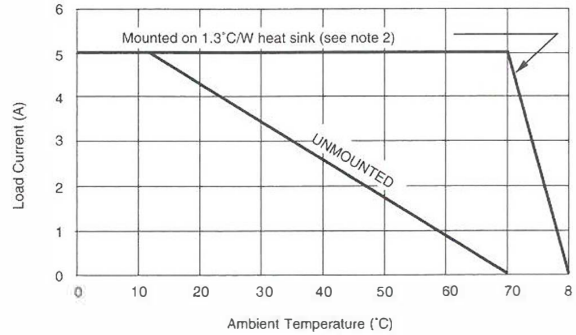
Figure 4 – 603-2 load current vs. temperature
