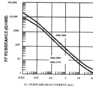
Figure 3. Typical RF Resistance vs. Forward Bias Current.
