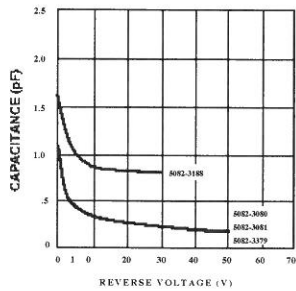
Figure 5. Typical Capacitance vs. Reverse Voltage.
