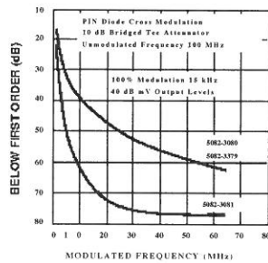
Figure 8. Typical Cross Intermodulation Distortion.
