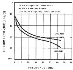
Figure 7. Typical Second Order Intermodulation Distortion.
