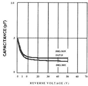
Figure 4. Typical Capacitance vs. Reverse Voltage.
