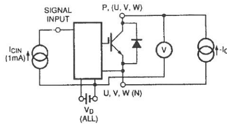
Figure 3 V_{EC} Test
