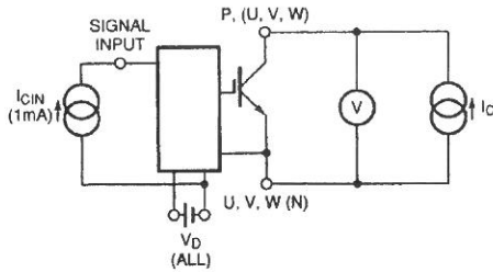
Figure 1 V_{CES} Test
