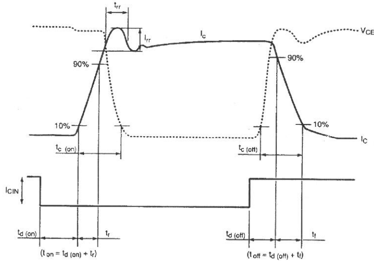
Figure 5 Switching Test Waveform
