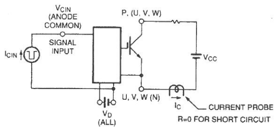
Figure 7 Over Current and Short Circuit Test
