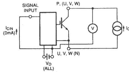
Figure 2 V_{CE(SAT)} Test
