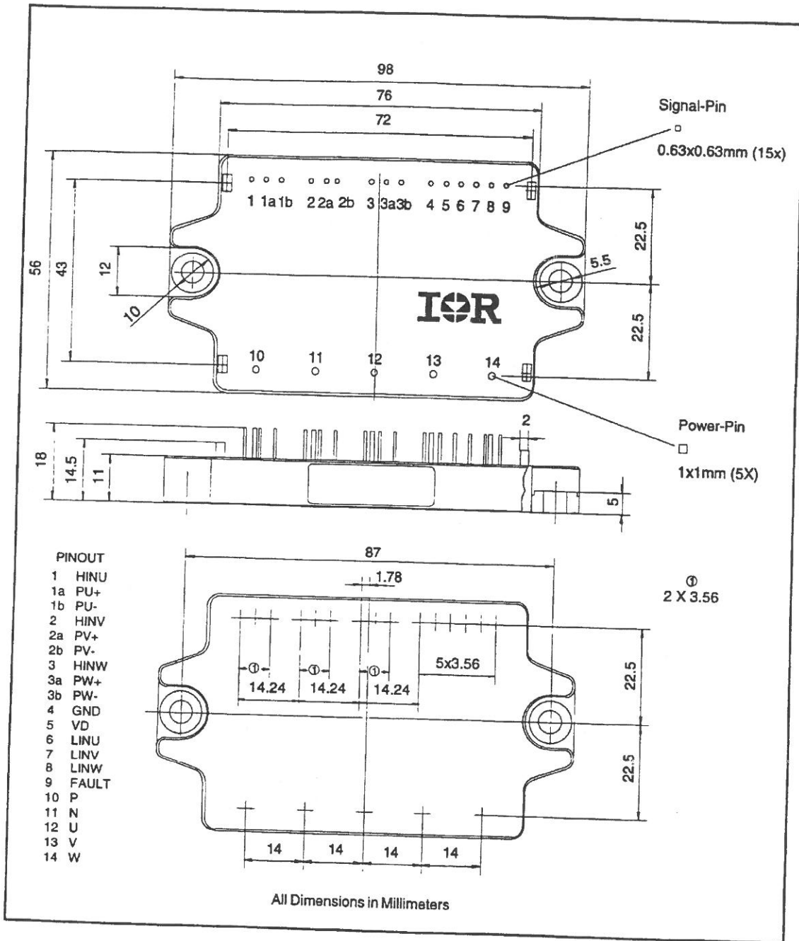
Fig. 7 - Package Outline
