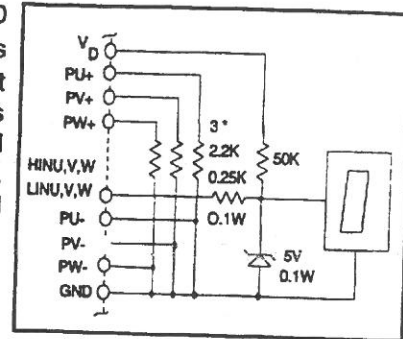
Figure 8 : Input Stage
