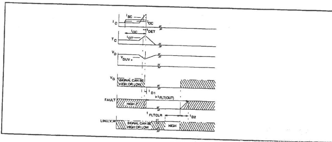
Fig. 10 - Timing Diagram
