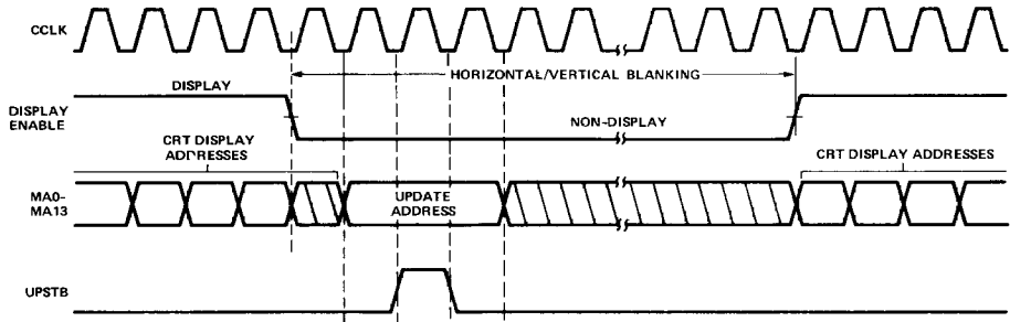
Figure 9. Retrace Update Timings
