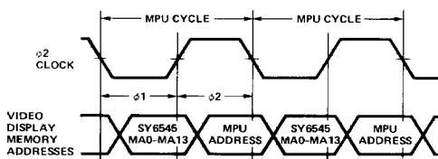
Figure 7. \phi 1/\phi 2 Interleaving
