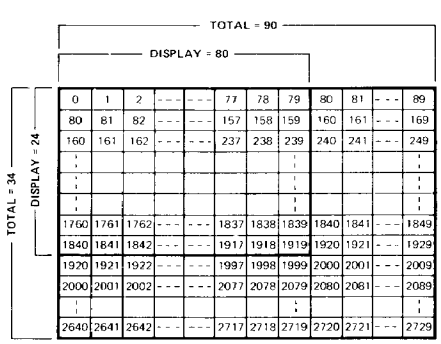
STRAIGHT BINARY ADDRESSING SEQUENCE
