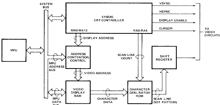
Figure 5. Shared Memory System Configuration
