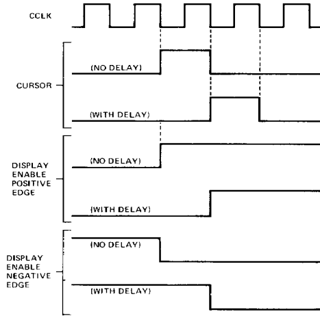
Figure 10. Cursor and Display Enable Skew
