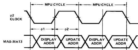
Figure 8. \phi 1/\phi 2 Transparent Interleaving
