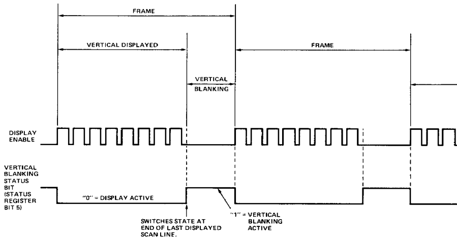
Figure 11. Operation of Vertical Blanking Status Bit
