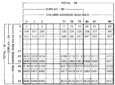
ROW/COLUMN ADDRESSING SEQUENCE
