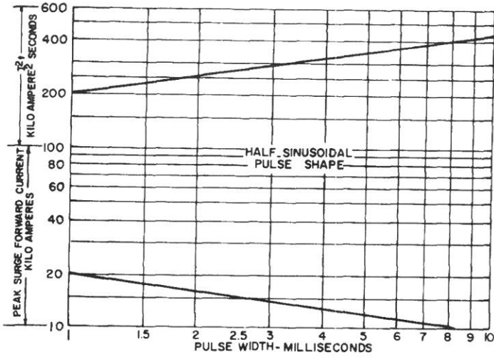
7. SUB CYCLE SURGE AND I^2t RATING FOLLOWING RATED LOAD CONDITIONS
