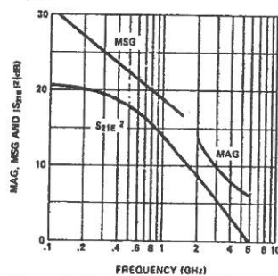
Figure 2. Typical MAG, Maximum Stable Gain (MSG) and |S 21E | 2 vs. Frequency (V CE = 18 V, I C = 30 mA), for the HXTR-5101.
