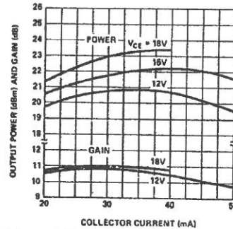
Figure 6. Typical P 1dB and Associated 1 dB Compressed Gain vs. Collector Current at 2 GHz, for the HXTR-5103.
