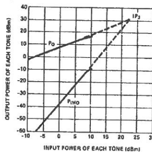
Figure 12. Typical Two Tone Third Order Intermodulation Distortion at 2 GHz for a Frequency Separation of 5 MHz ( V_{CE} = 18V , I_C = 30mA ) for the HXTR-5101.
