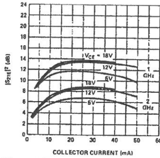
Figure 8. Typical IS_{21P}^2 vs. Collector Current at 1 and 2 GHz, for the HXTR-5103.
