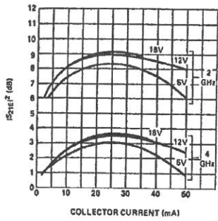
Figure 7. Typical IS_{21P}^2 vs. Collector Current at 2 and 4 GHz, for the HXTR-5101.
