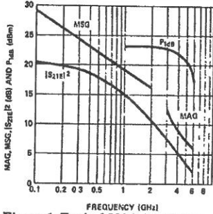
Figure 1. Typical MAG, Maximum Stable Gain (MSG), |S 21E | 2 and P 1dB Linear Power vs. Frequency (V CE = 18 V, I C = 30 mA), for the HXTR-5001.
