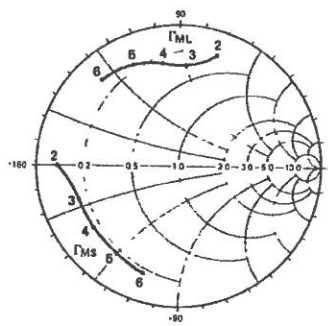
Figure 14. Typical \Gamma_{MS} , \Gamma_{ML1} (Calculated From the Average S-Parameters) in the 2 to 6 GHz Frequency Range ( V_{CE} = 18V , I_C = 30mA ), for the HXTR-5101.
