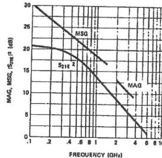
Figure 3. Typical MAG, Maximum Stable Gain (MSG), and |S 21E | 2 vs. Frequency (V CE = 18 V, I C = 30 mA), for the HXTR-5103.
