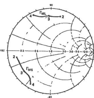
Figure 15. Typical \Gamma_{MS} , \Gamma_{ML1} (Calculated From the Average S-Parameters) in the 2 to 4 GHz Frequency Range ( V_{CE} = 18V , I_C = 30mA ), for the HXTR-5103.
