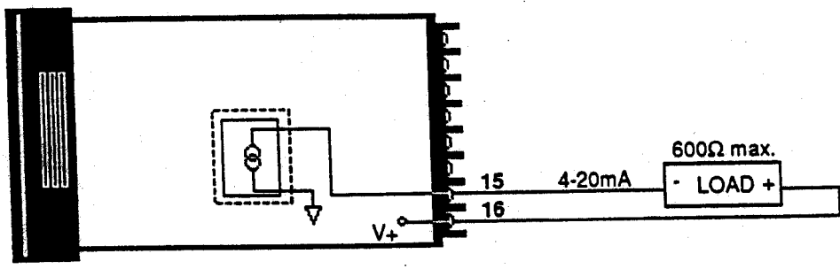
Figure 16 - 4-20mA, Output 1 Wiring
