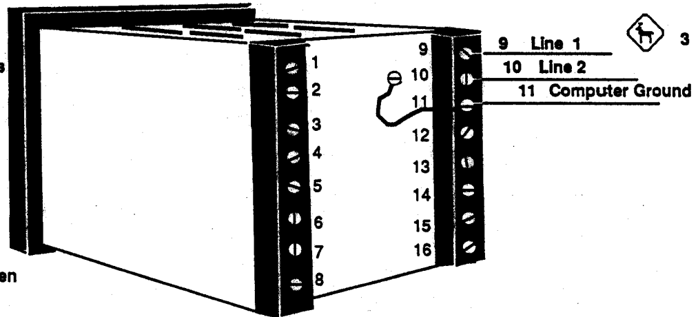
Figure 23 - Power Wiring
