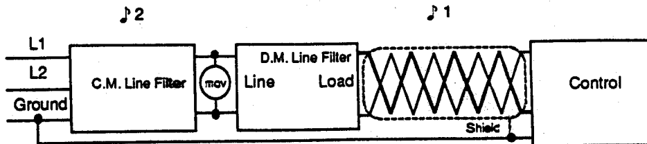
Figure 7 - Combination Differential/Common Mode Filter Wiring
