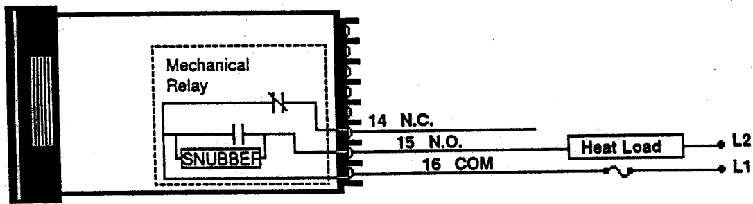
Figure 14 - Mechanical Relay, Output 1 Wiring
