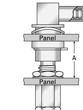
Right angle float-mounted cable plug (7335 series) and straight bulkhead cable jack (7303 series):
