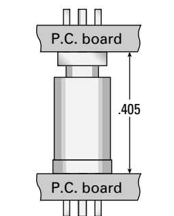
Straight P.C. board plug (7225 series) and straight P.C. board jack (7209 series)
