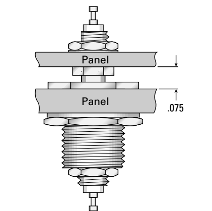
Straight bulkhead jack receptacle (7219 series) and recessed bulkhead jack receptacle (7496 series)
